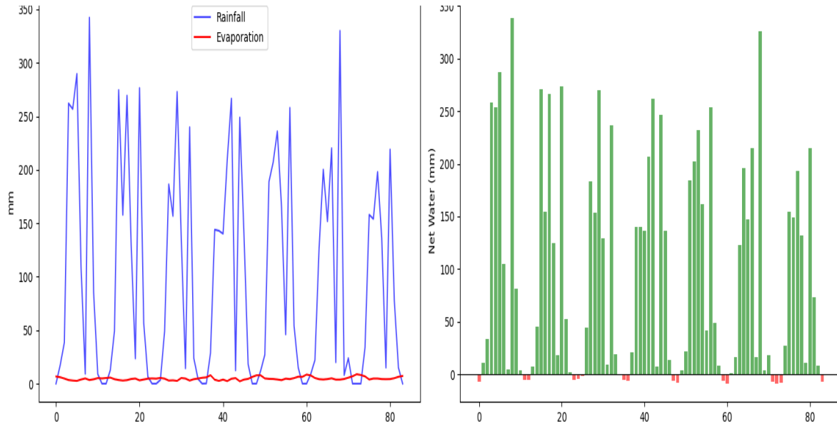
Figure 2: Monthly rainfall and evaporation and hydrological balance (P – E), 1990–2025.
