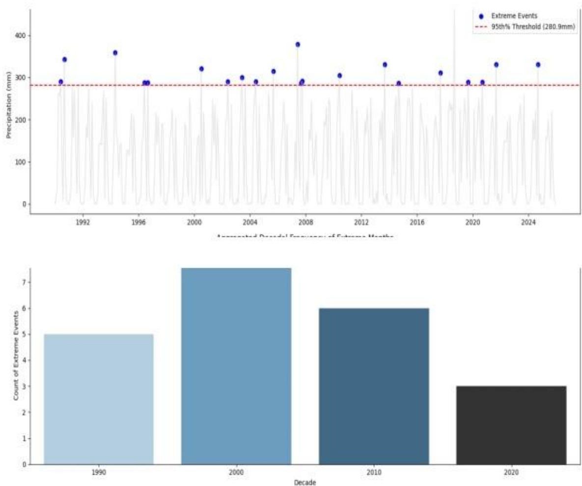
Figure 4: Chronological distribution and decadal frequency of extreme rainfall months (>280.9 mm month -1 ), 1990–2025.
