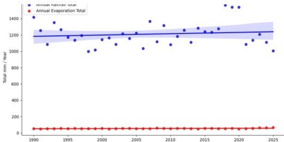
Figure 6: Annual rainfall and evaporation totals, 1990–2025.
