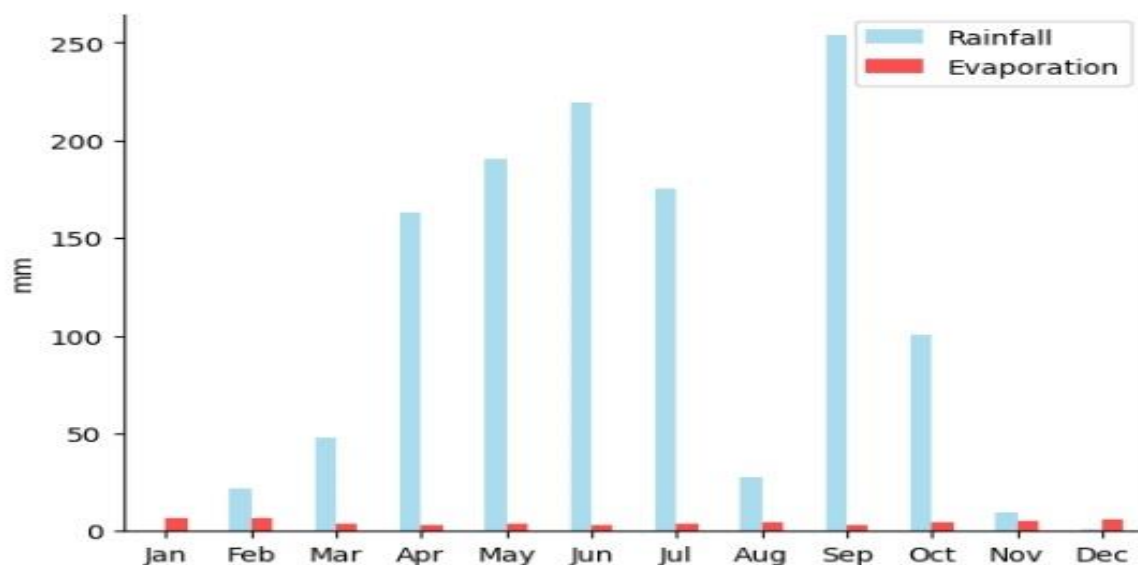
Figure 7: Mean monthly rainfall and evaporation, 1990–2025.
