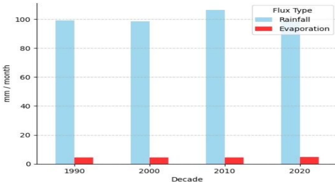
Figure 8: Decadal mean rainfall and evaporation, 1990–2025.
